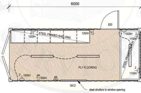
20' WORKSHOP SCALE 1:50
